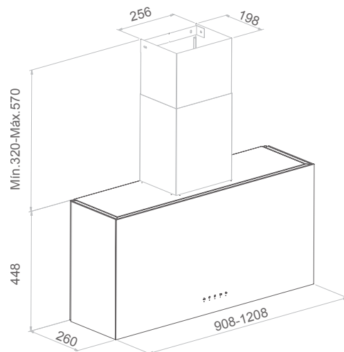
Dimensions in mm Special Custom-Made Flues Flue included as standard with the ducted version
