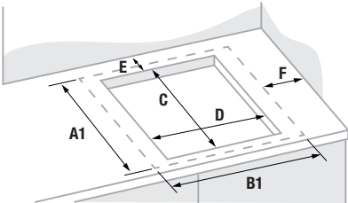
Above-Worktop Glass Installation
