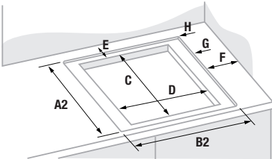
Flush-Mounted Glass Installation
